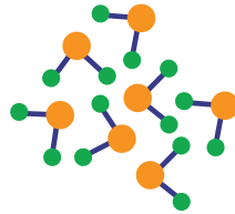
cold water molecules
